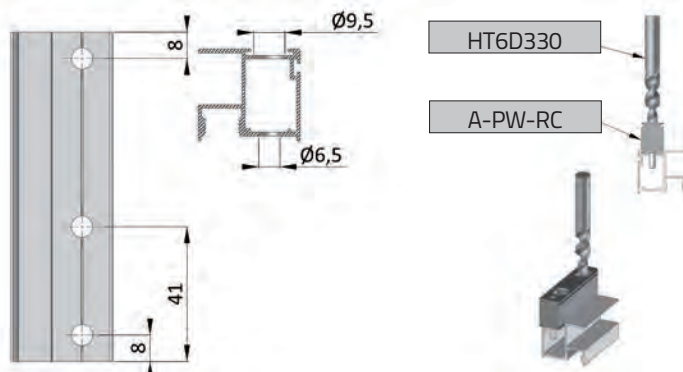
Arrangement of fixing holes
